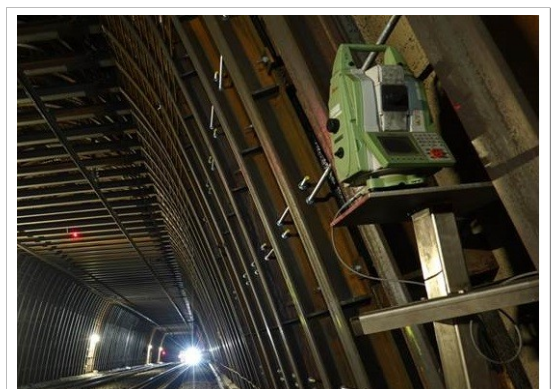
Figure C: Tachymeter measuring position of crossbar.
