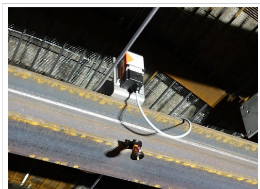
Figure B: Dimetix D-Series Sensor mounted on crossbar.
