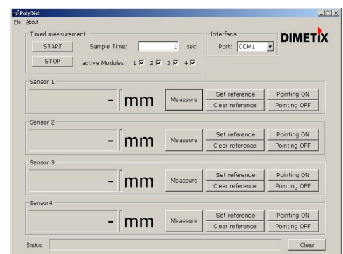
Fig 2: User interface of PolyDist
